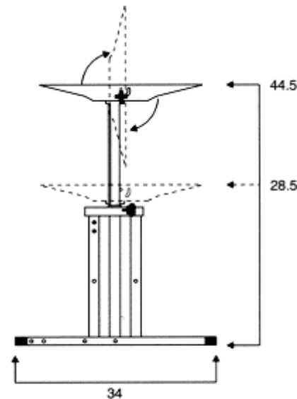
XJ-5A Pedestal
